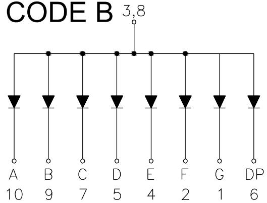
Common Anode
