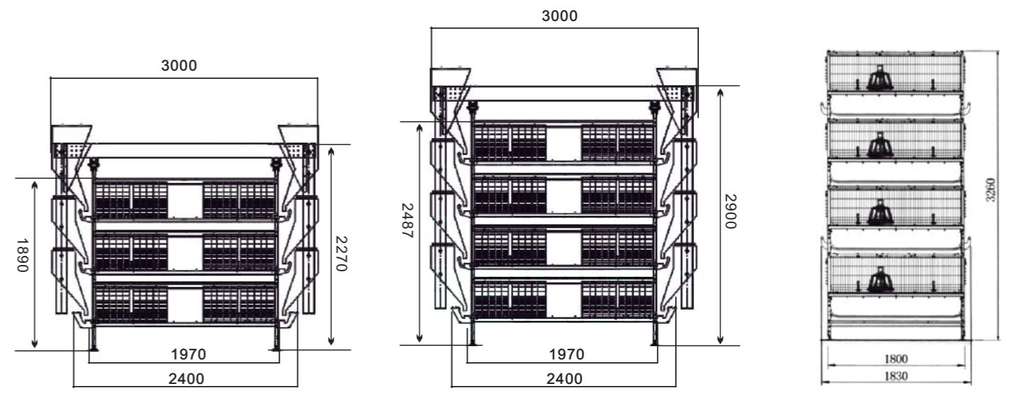
3 Tier Manual Load Cage
