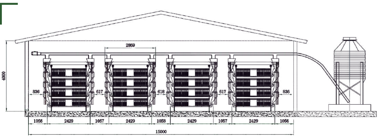
H Type Cage with Auto System
