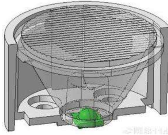
Led Lens
