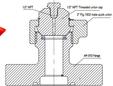
1 13/16" 15,000 PSI x 2" Fig. 1502 Male(Nut Half). API 6A (Shown Above)
