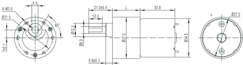
Gear Motor Dimensions (mm)
