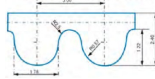
HTD-3M型(节距PITCH=3.00mm)
