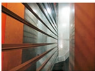
Aluminum profile powder coating line
