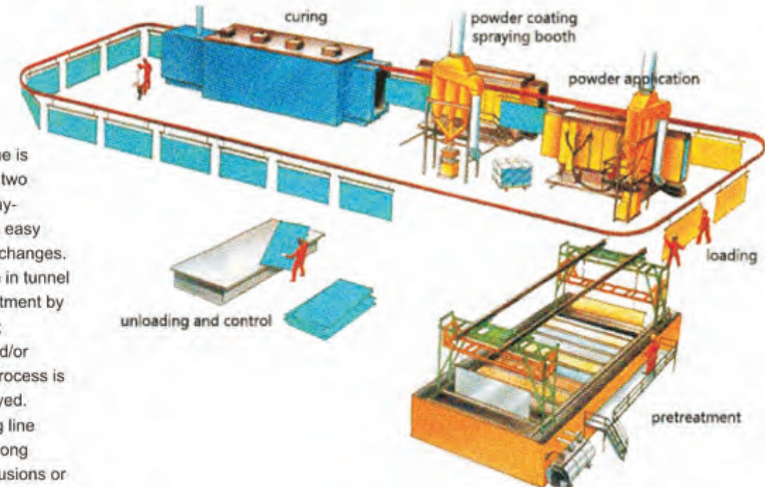
Powder Coating Line with DIP-Pre-treatment
