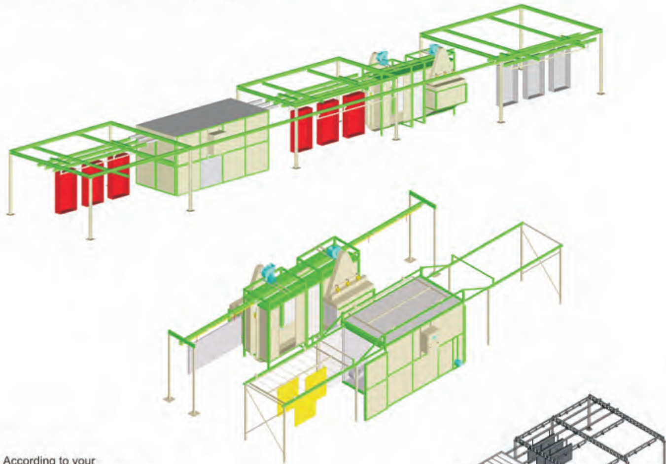
Powder coating set with head-up transport system
