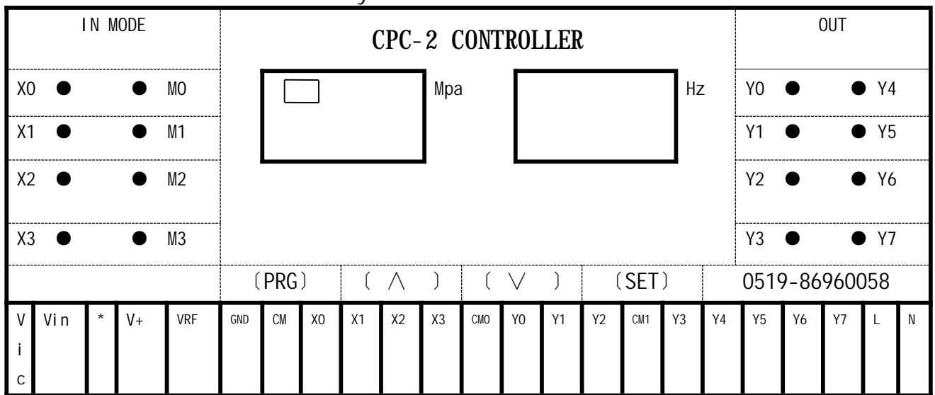
Panel layout and terminal
