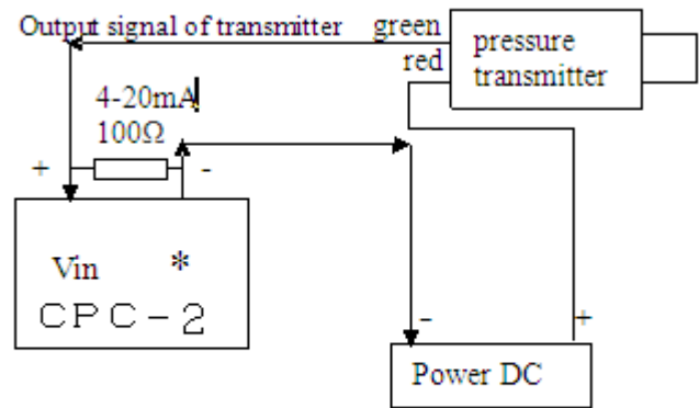
the connection of two-wire system transmitter
