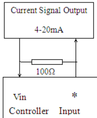
the external input of the controller the connection of current signal
