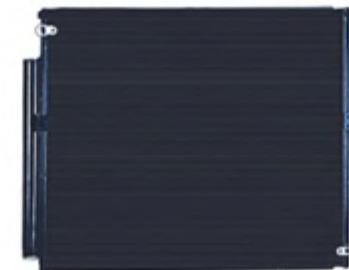
MODEL:TOYOTA LAMD KING DOUBLE GRJ120 2003 OEM:884 616 0090 DPI:3288 LENGTH:635 HEIGHT:540 THICKNESS:16
