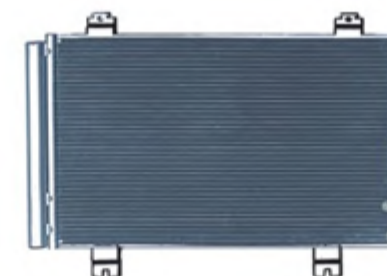
MODEL:TOYOTA CROWN OEM:884 600 N010 LENGTH:690 HEIGHT:412 THICKNESS:16
