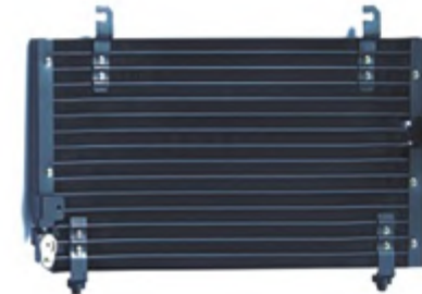
MODEL:TOYOTA TERCEL 1995-1997 OEM:884 601 6340 DPI:4668 LENGTH:750 HEIGHT:310 THICKNESS:22
