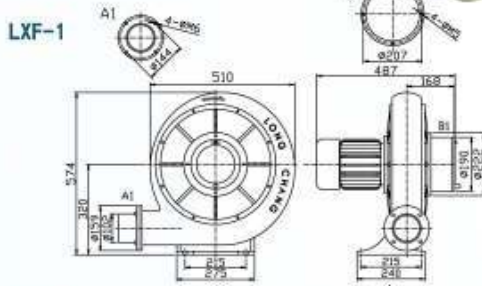
(A) 消音入風口 Muffler Inlet
