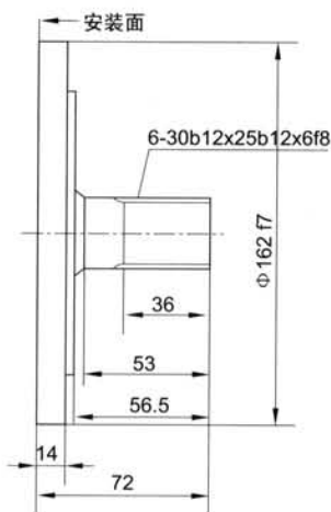
JMDG2-**T12
