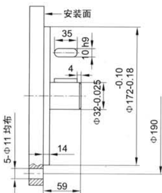
JMDG2-**T12
